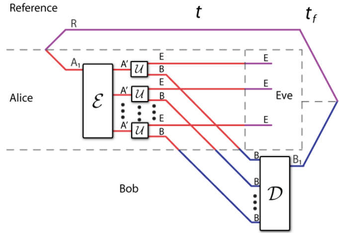
Figure 1: The most general protocol for quantum communication (or, equivalently, entanglement generation). Alice performs an encoding on her A_1 system and then feeds the outputs of the encoder into the inputs of the channels. Bob receives all of the channel outputs and performs some decoding map. If the protocol is good, at the end, Alice and Bob should share a state that is arbitrarily close in trace distance to a maximally entangled state.
