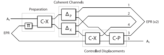
FIG. 1. Coherent teleportation. \pi is a reflection operation. C-X and C-P are a controlled-position displacement and a controlled-momentum displacement respectively.
