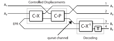
FIG. 3. Coherent superdense coding implements two conat channels.
