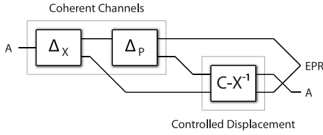
FIG. 2. Alternate coherent teleportation protocol.
